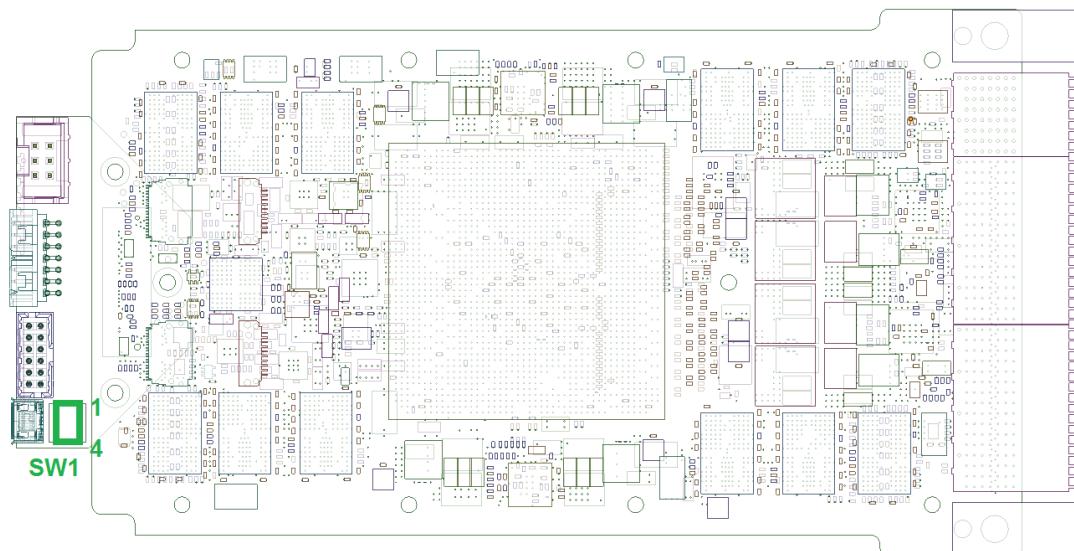
Figure 6 : Switches
