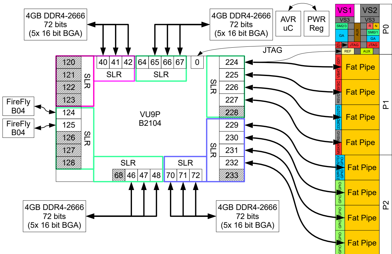
Figure 3 : ADM-VPX3-9V2 VU9P Block Diagram
