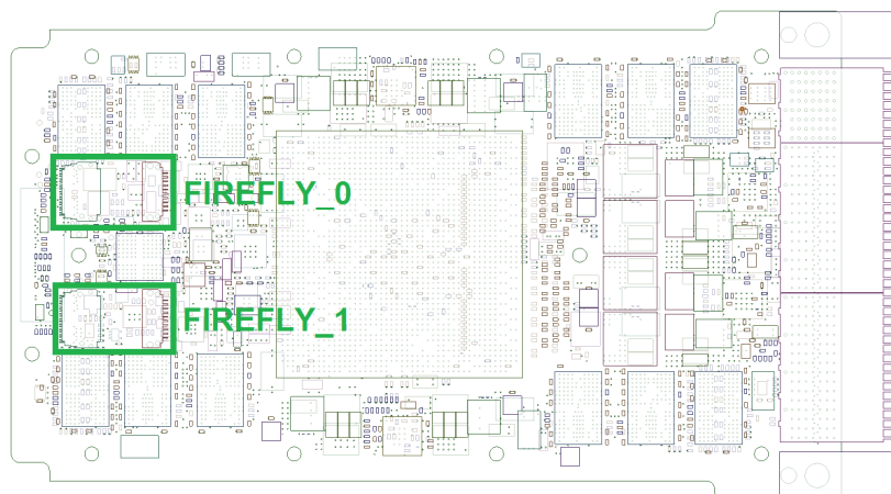
Figure 9 : FireFly Location
