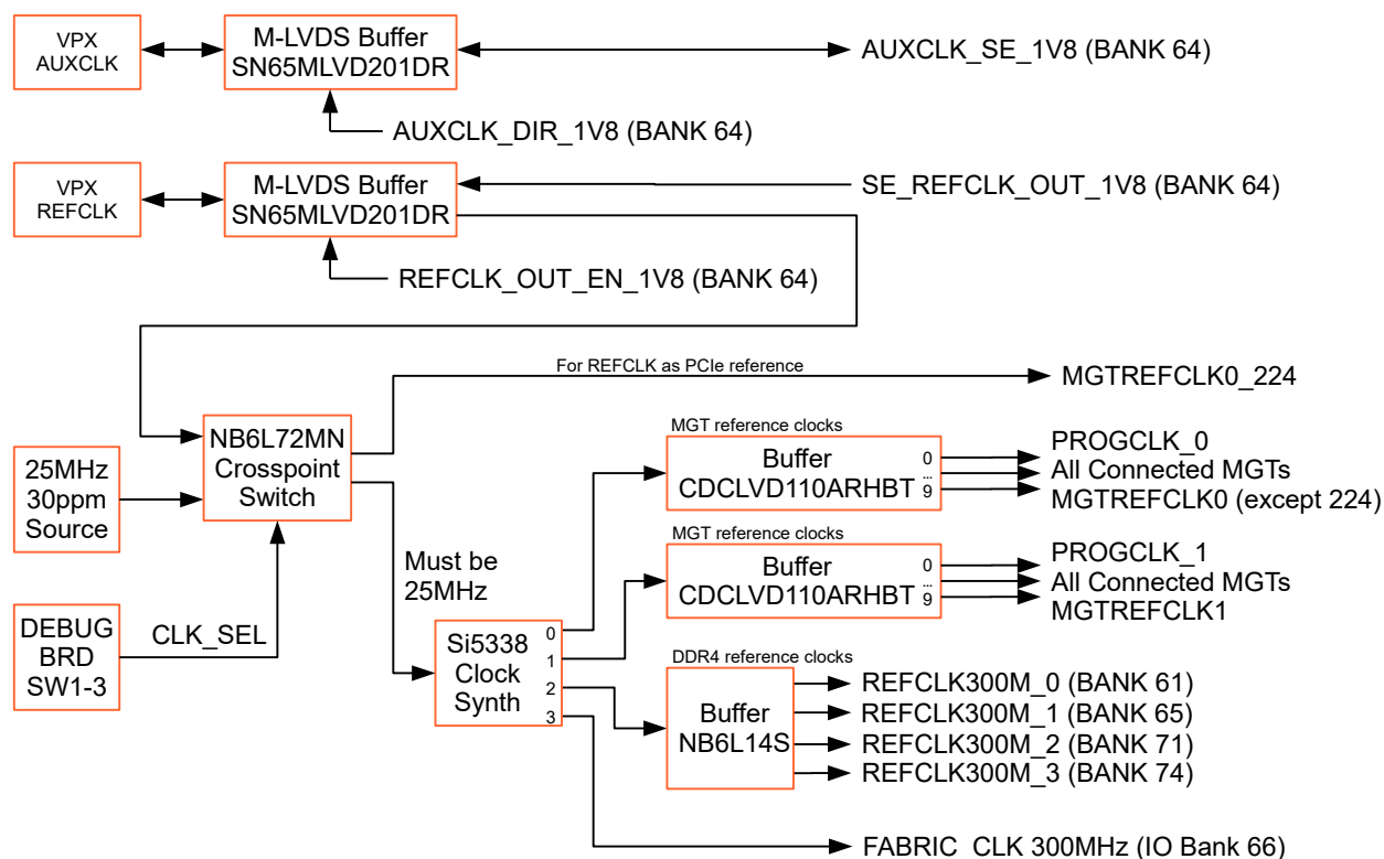
Figure 8 : Clock Topology
