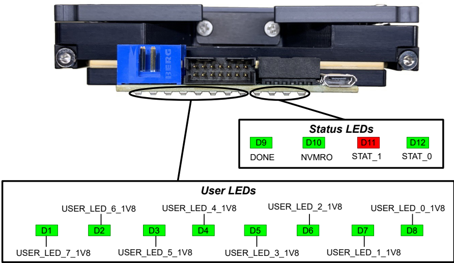
Figure 7 : Front Panel LEDs
