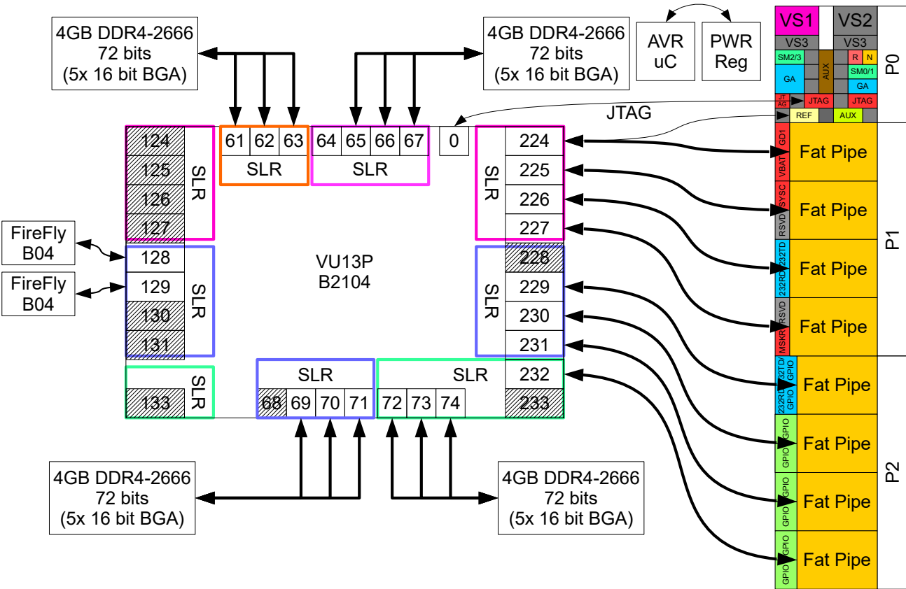
Figure 4 : ADM-VPX3-9V2 VU13P Block Diagram
